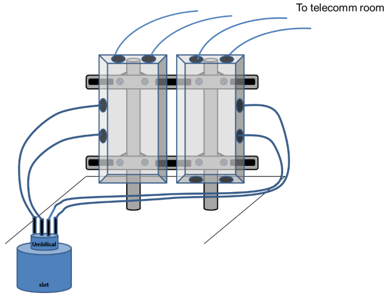
Typical arrangement
